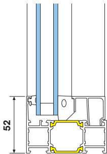
Karm
